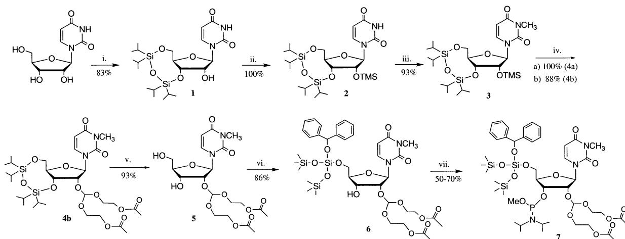
Scheme 1. (i) TIPDSCl 2 , pyridine, 0 °C→rt; (ii) TMSCl, Et 3 N, CH 2 Cl 2 , 0 °C→rt; (iii) N,N -dimethylformamide dimethylacetal (DMF-DMA), benzene, reflux; (iv) (a) pTSA-H 2 O, Et 3 N, THF; (b) tris(2-acetoxyethoxy)orthoformate, pyridinium p -toluenesulfonate, 4-( tert -butyldimethylsilyloxy)-3-penten-2-one, dioxane, rt for 48 h; (v) TMEDA-HF, CH 3 CN, 0 °C; (vi) BzH-Cl, diisopropylamine, CH 2 Cl 2 , 0 °C; (vii) methyl tetraisopropyl phosphoradimidate, 4,5-dicyanoimidazole, CH 2 Cl 2 , rt.
