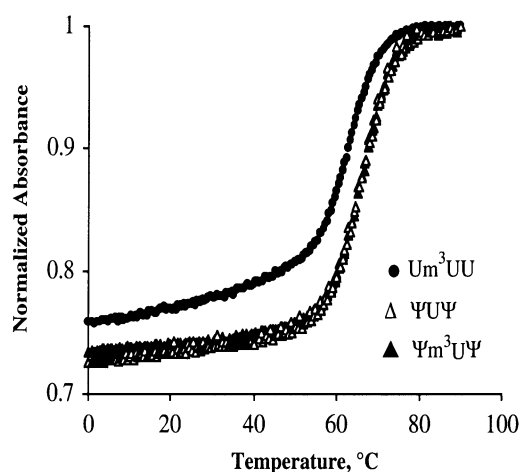
Figure 2. Representative normalized UV melting curves for the modified RNAs taken in 15 mM NaCl, 20 mM sodium cacodylate, 0.5 mM EDTA, pH 7.0 are shown. The melting curves were obtained using an Aviv 14DS UV-vis spectrometer. The curves for singly modified RNA (Um 3 UU), pseudouridine-modified RNA (ΨUΨ), and triply modified RNA (Ψm 3 UΨ) are represented by closed circles, open triangles, and closed triangles, respectively. The melting curves were normalized at 95°C.
