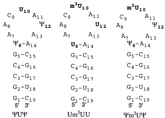
Figure 1. The structures of 3-methyluridine (m 3 U) and pseudouridine (Ψ) are shown. Secondary structure representations of the synthetic RNAs are based on the 1920-hairpin region (helix 69) of E. coli 23S rRNA (nucleotides G 1906 to C 1924 ). The nucleotide positions have been renumbered consecutively from G 1 to C 19 . Positions 6 (1911), 10 (1915), and 12 (1917) are modified with m 3 U or Ψ.
