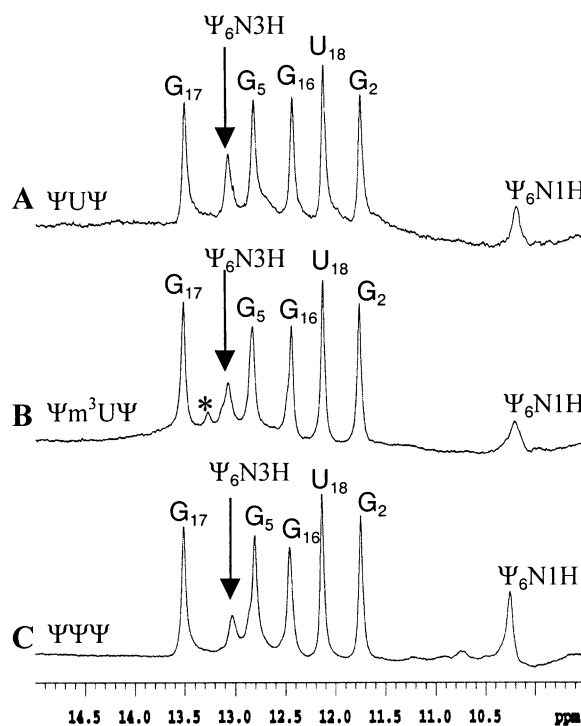
Figure 5. The 1D imino proton (guanine N1H/uridine N3H/pseudouridine N1H and N3H) NMR spectra for RNAs ΨUΨ (A), Ψm 3 UΨ (B) and ΨΨΨ (C) are shown. The experimental conditions were the same as those described in Figure 4. The spectrum in panel C was assigned previously 8 and is shown here for comparison.
