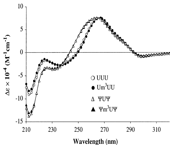
Figure 3. CD spectra of the unmodified and modified RNAs taken on a Jasco J600 spectropolarimeter from 210 to 320 nm at ambient temperature in 15 mM NaCl, 20 mM sodium cacodylate, 0.5 mM EDTA, pH 7.0 are shown. The molar ellipticities were normalized to RNA concentration (4.9, 7.4, 3.2, and 3.6 × 10 -6 M in molecules of RNA for UUU, Um 3 UU, ΨUΨ, and Ψm 3 UΨ, respectively) based on an extinction coefficient of 188,860 cm -1 M -1 for all RNAs and A 260 values at 90 °C. The spectra for unmodified (UUU), singly modified (Um 3 UU), pseudouridine-modified (ΨUΨ), and triply modified (Ψm 3 UΨ) RNAs are represented by open circles, closed circles, open triangles, and closed triangles, respectively. Each spectrum is the average of four scans. The spectrum for UUU was obtained previously 8 and is shown here to allow for direct comparison to Um 3 UU.
