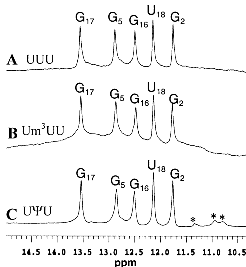
Figure 4. The 1D imino proton (guanine N1H/uridine N3H/pseudouridine N1H and N3H) NMR spectra obtained at 3 °C on a Varian UNITY 500MHz spectrometer in 30 mM NaCl, 10 mM sodium phosphate, 0.5 mM Na 2 EDTA, pH 6.5 (90% H 2 O/10% D 2 O) are shown. The RNA concentrations for UUU (A), Um 3 UU (B), and UΨU (C) were 0.8 to 1 mM. Nucleotide assignments based on the 1D-NOE difference spectroscopy (data not shown) are indicated above each resonance with the nucleotides numbered consecutively from G 1 to C 19 . The spectra in panels A and C were assigned previously 8 and are shown here to allow for direct comparison to Um 3 UU.
